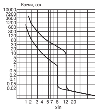
BA88-39, 500-630 A
