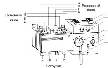
16-630 A
