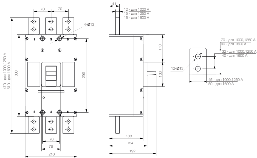
BA88-43
