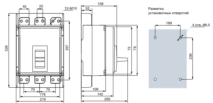
E2KR-16P (800-1600 A)
