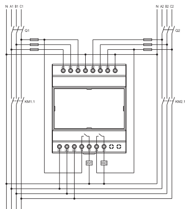
ETS-2ZC
