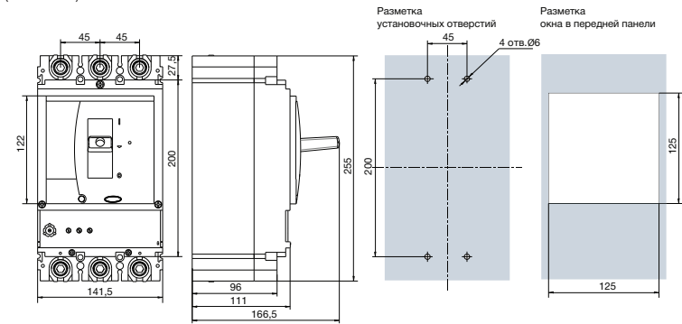
E2KR-16P (800-1600 A)
