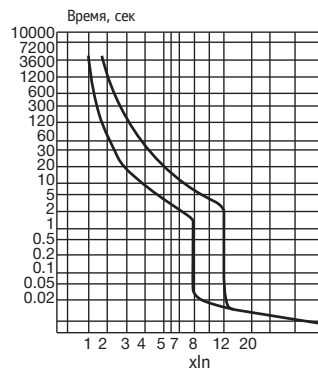
BA88-41, 800 A
