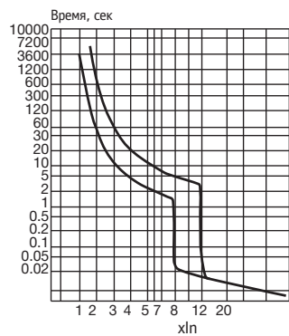
BA88-43, 1000-1600 A
