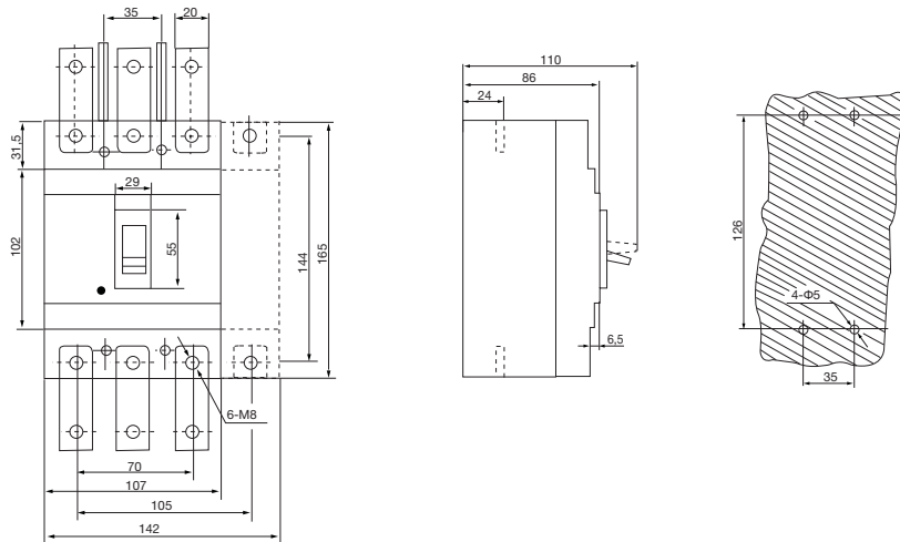
BA88-35
