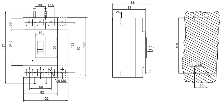
BA88-31
