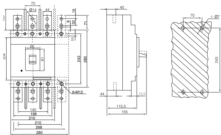
BA88-41
